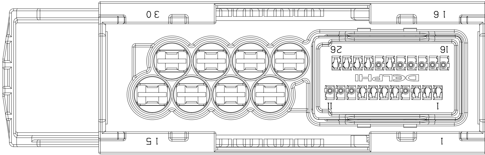
TYPE 102 SAME AS TYPE 101 EXCEPT AS SHOWN
