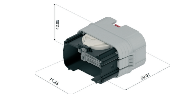
ErgoMate™ 38W Female
