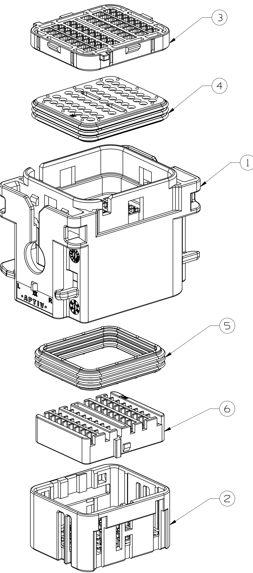
EXPLODED VIEW
