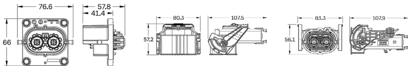
Header Connector
